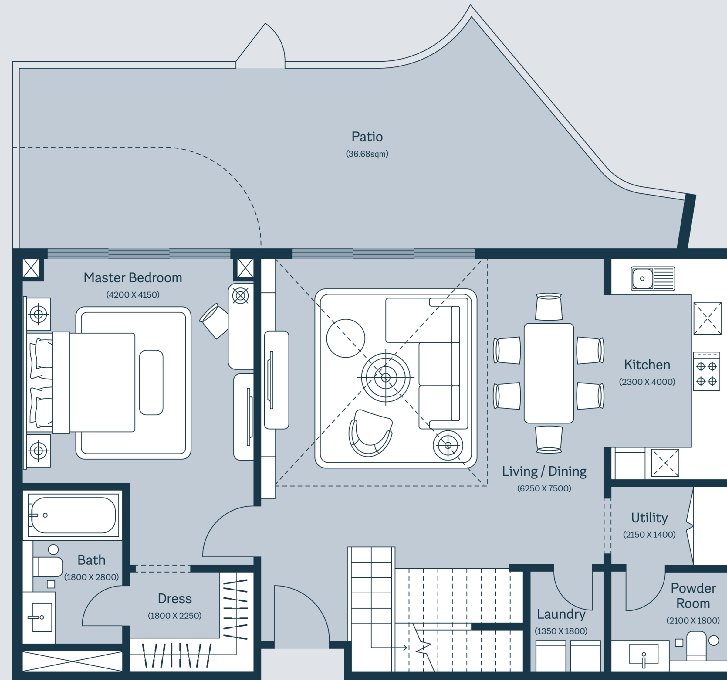
Ground Floor
