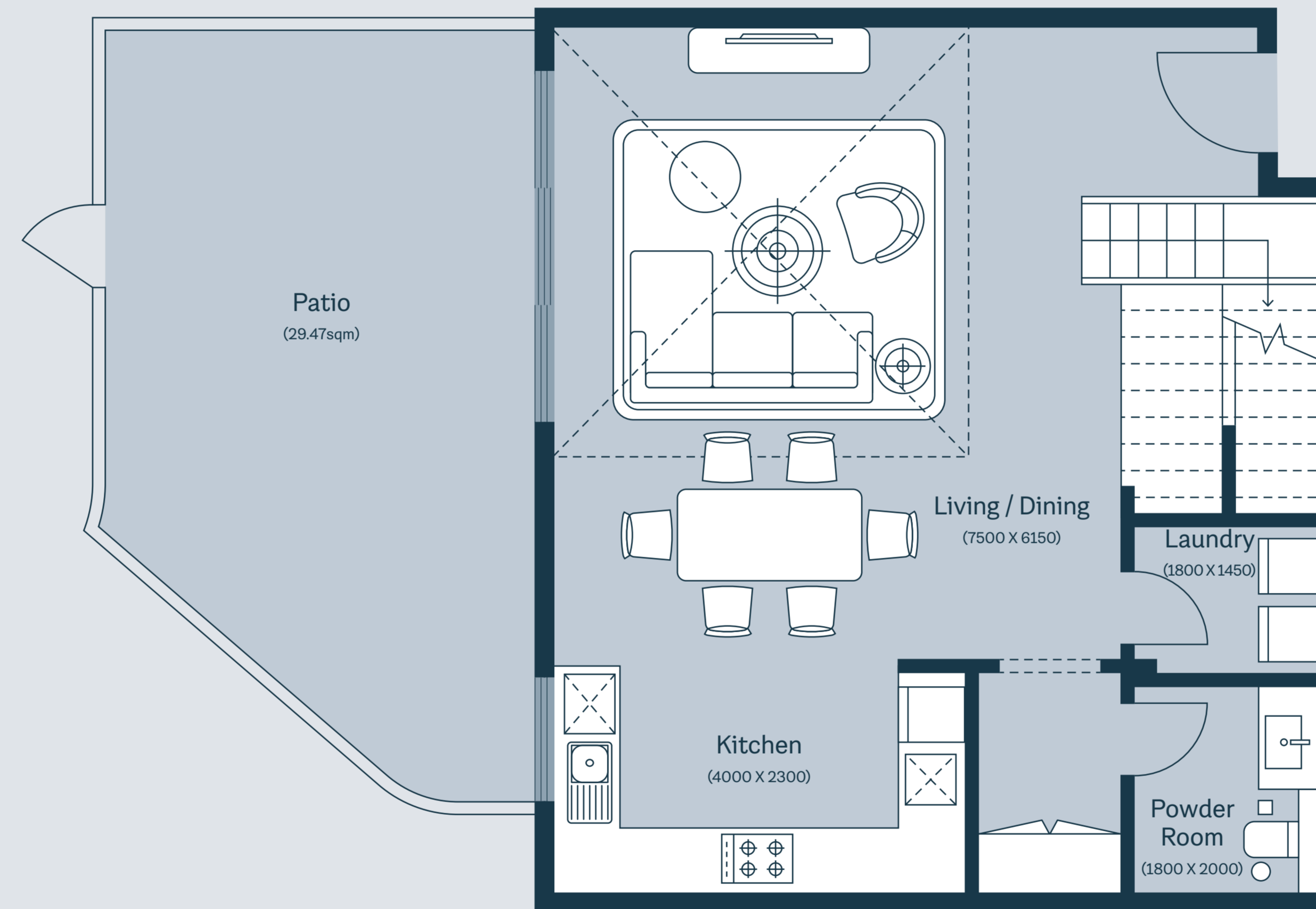
Ground Floor
